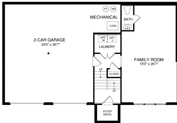
LOWER LEVEL/ FOUNDATION PLAN
